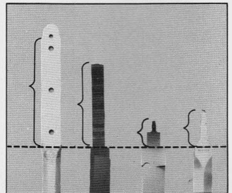
The main strength—or weakness—of a knife is revealed when the grip is removed. Compare the full tang of the Ek (L) to the smaller "stub" tangs of the other well-known, yet weaker, knives.
