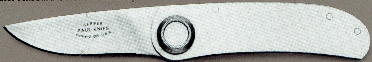
MODEL 2P STAINLESS STEEL #8001 2½" drop-point blade. Brushed stainless steel handle is easily personalized. Length open, 6"; closed 3½". Blade thickness, .115".
