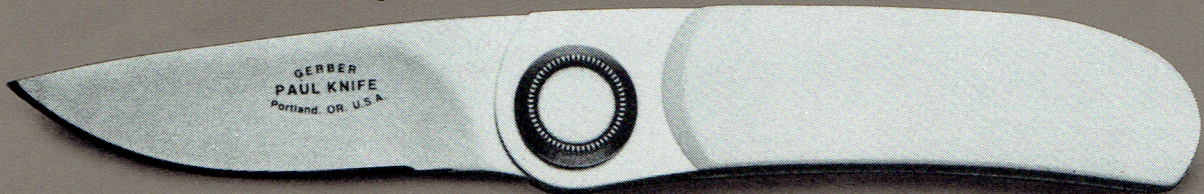
DELUXE MODEL 2PM #8011 Ivory colored onlays. 2½" drop-point blade. Length open, 6"; closed, 3½". Blade thickness, .115".
