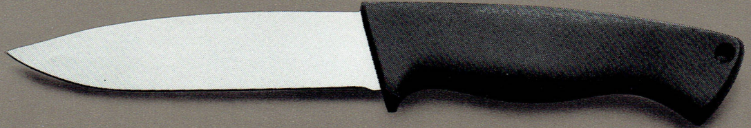
A-475 #5221 4¾" drop-point blade, designed for large game. High speed tool steel. Length, 9¾". Blade thickness, .100". Scabbard included.
