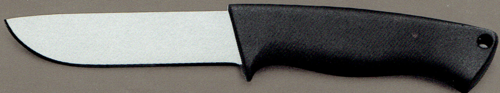
A-425 #5211 4¼" utility skinning blade. High speed tool steel. Perfect for camping and field dressing. Length, 8¾". Blade thickness, .100". Scabbard included.
